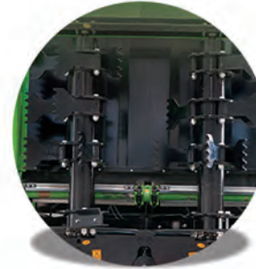
Çift tepsili ve tokatlamalı dağıtıcı sistem Twin-tray and threshing distributor system
